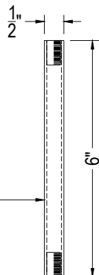
Stem, \frac{1}{2}'' \text{Ø} \times 6'' \text{L} \times \frac{1}{8}'' \text{IPS} (Optional, additional stem if necessary)
