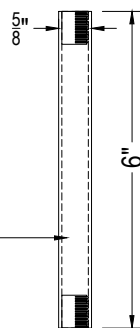
Stem, \frac{5}{8} " \varnothing x 6"L x 1/4 IPS (Optional, additional stem if necessary)
